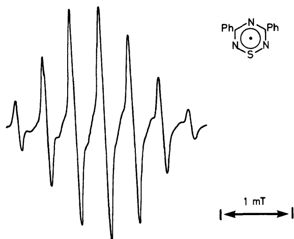
Figure 2. E.s.r. spectrum of (\text{Ph}_2\text{C}_2\text{N}_3\text{S})^\cdot ( 2 ) in methylene dichloride.
